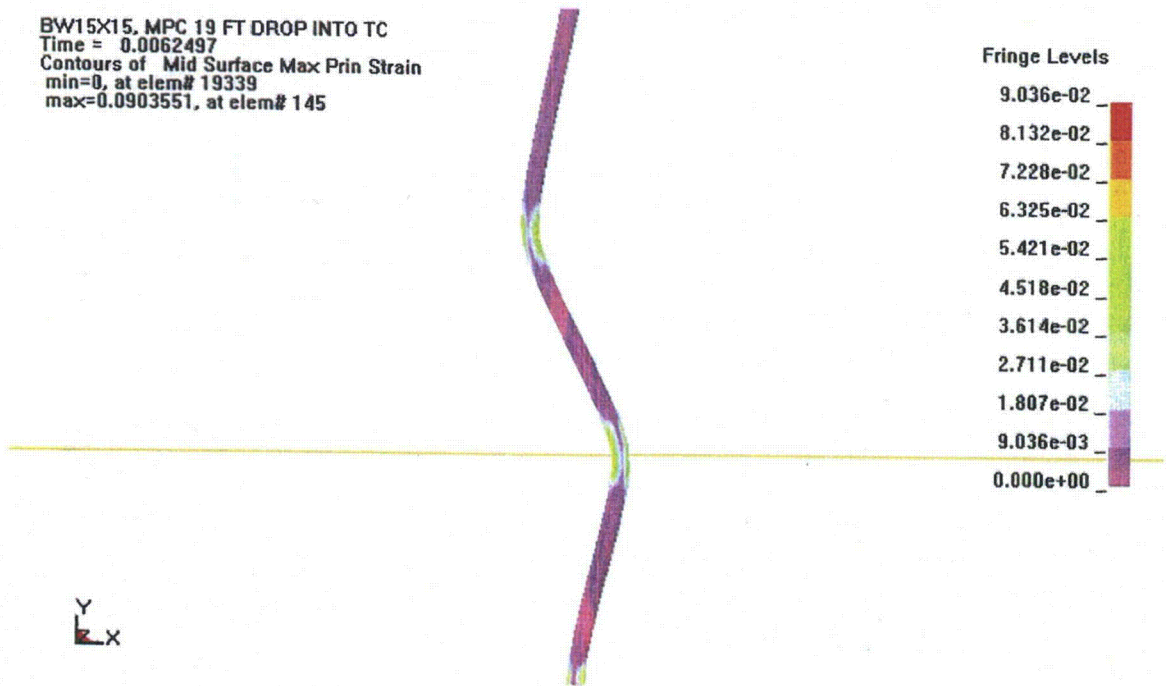
Figure C.17. Maximum Principal Strain at Time of Maximum Response (19-Foot Drop)
