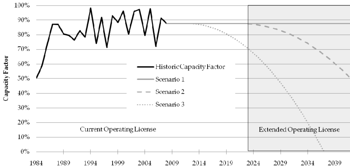
Figure 39: Estimated Electricity Production at SONGS
